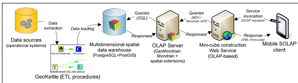
Fig. 3. Architecture of the Web service for SOLAP mini-cube delivery [17]
