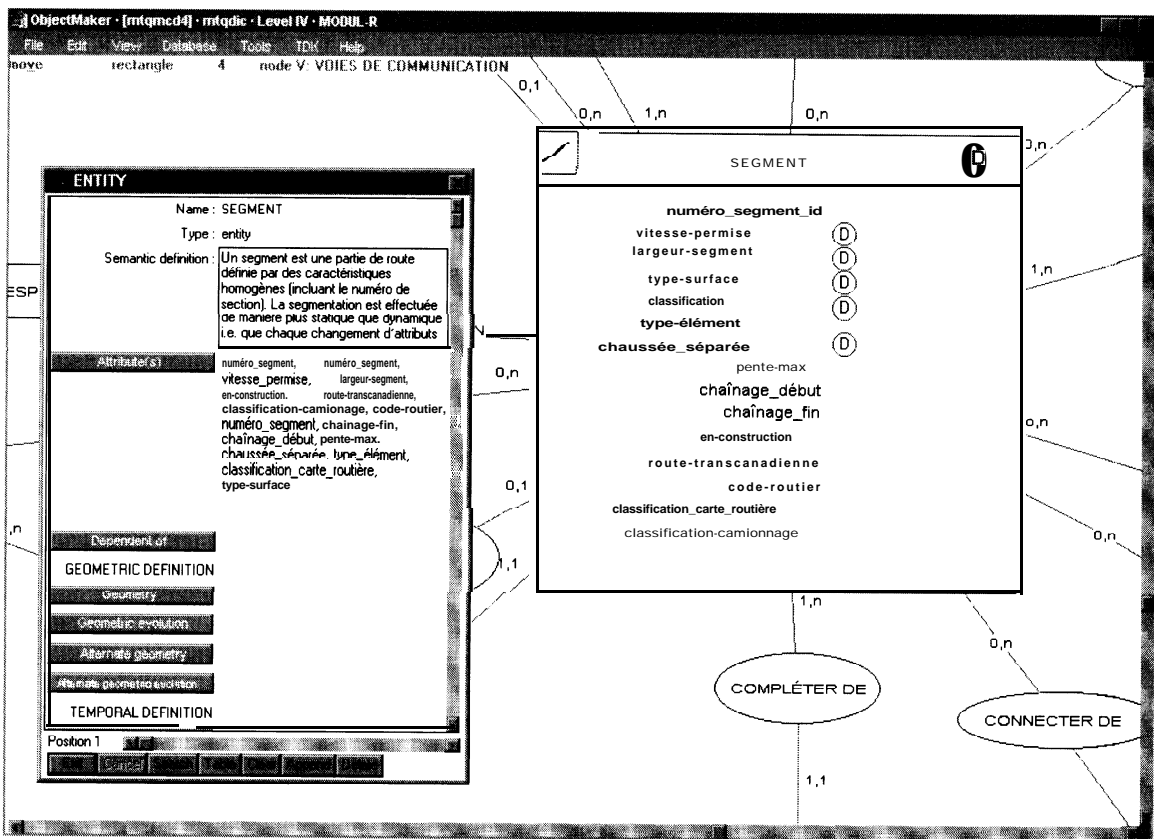
Fig 7. Example of a screen display of the working prototype Orion built with the Object Maker metaCASE; it shows an extended entity/relationship analysis model with spatial and temporal pictograms, as well as an extract of the extended data dictionary which is partly filled automatically from the schema; it is used for automatic code generation for Intergraph GIS.
