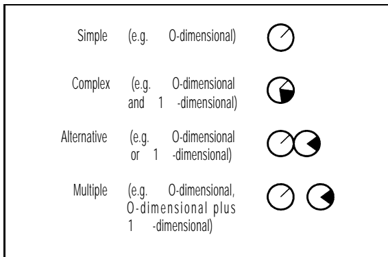
Fig 5. Graphical notation used for temporal patterns; an example of a spatio-temporal pattern is also presented, that is one of a 0-dimensional object (e.g. an emergency vehicle) with a position which sometimes varies continuously and sometimes remains stable.
