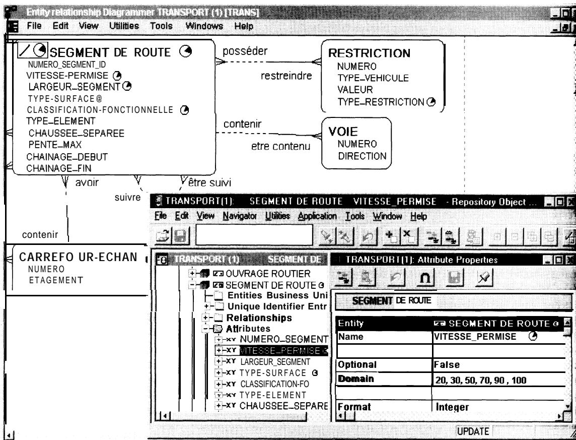
Fig 2. Extract of an analysis model made with Oracle Designer 2000 (Oracle Corporation 1996) where spatial and temporal pictograms (see Figures 4 and 5) are added to indicate the geometry and temporality of geographical features (model in development for Quebec Ministry of Transportation at the time of writing the present chapter).
