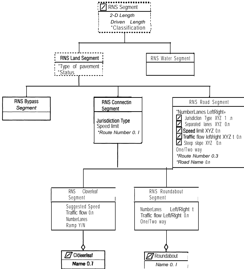
Fig 3. Extract of an object model using spatial 'plug-ins' (Bédard and Sondheim 1996); see Figure 4 for explanation of pictograms.
